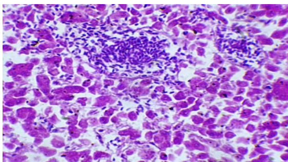
Figure 1: Section showed marked portal vein dilation with inflammatory edematous exudates as well as portal fibrosis was recorded with sever atrophy of adjacent parenchymal cell zone.
